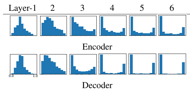
Figure 9: Histograms of the domain proportions of each layer in our domain mixing model for English-to-German Task. Within each histogram, 0 means pure News domain, and 1 means pure TED domain.
