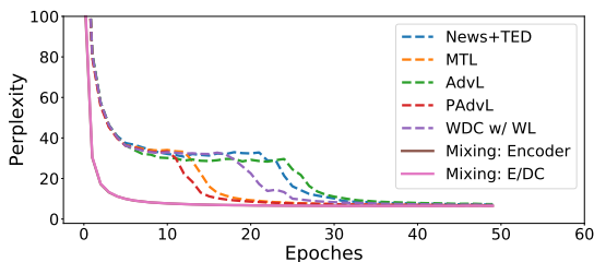
Figure 6: Perplexity v.s. Number of epochs for English-to-German.
