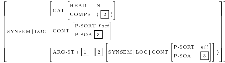
Figure 3: A partial description of the lexical entry of fact
