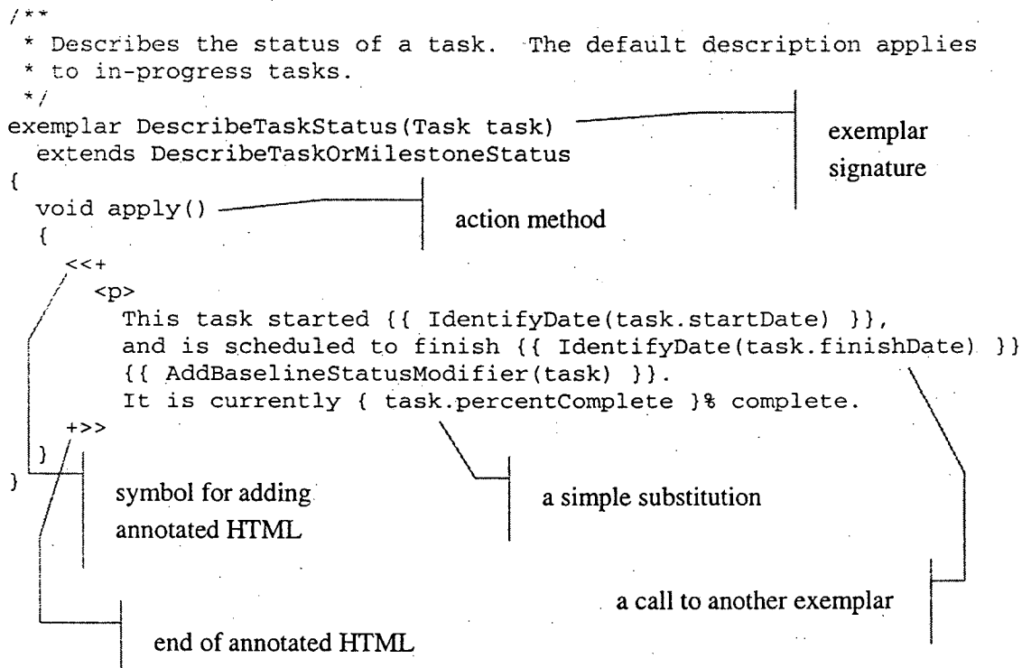
Figure 4: Exemplar describing the status of a task
