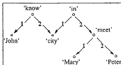
Figure 5 : SemS of (4)
