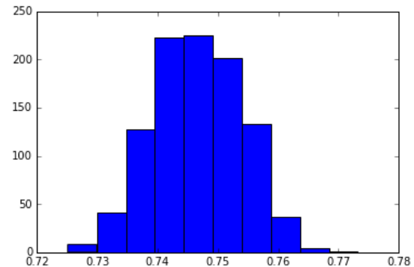
Figure 3: Confidence Interval for SMK Prompt model
