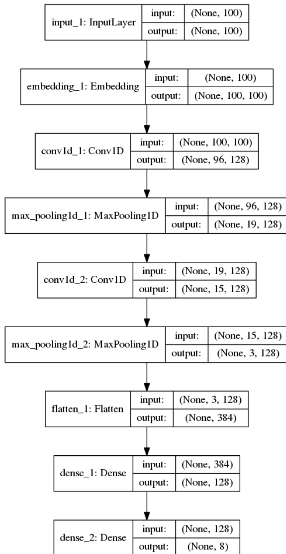
Figure 2: Convolutional Neural Network 6
