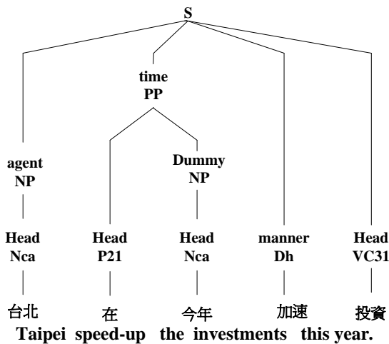
Figure 3: Parsed trees of “台北在印尼加速投資” and “台北在今年加速投資”
