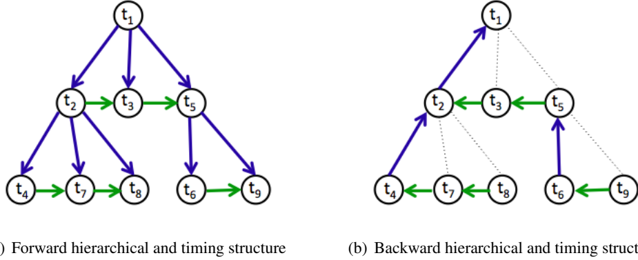
Figure 2: An example of model propagation in a graph-structured LSTM. Here, the node name are shown in a chronological order, e.g. comment t_1 was made earlier than t_2 . 2(a) Propagation of graph-structured LSTM in the forward direction. Blue arrows represent hierarchical propagation, green arrows represent timing propagation. 2(b) Backward hierarchical (blue) and timing (green) propagation of graph-LSTM.
