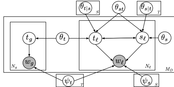
Figure 2: Plate notation for the proposed sense-topic model with all variables (except \alpha , the fixed Dirichlet hyperparameter used as prior for all multinomial distributions). Each instance has topic mixing proportions \theta_t and sense mixing proportions \theta_s . The instance set shares sense/topic parameter \theta_{st} , topic-sense distribution \theta_{s|t} , sense-topic distribution \theta_{t|s} , topic-word distribution \psi_t , and sense-word distribution \psi_s .
