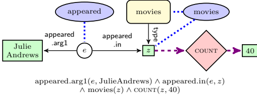
(b) Alternate Ungrounded Graph
