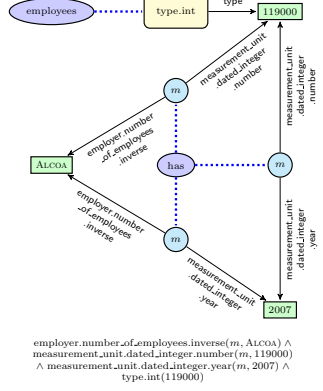
(b) Grounded Graph
