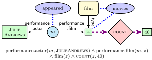
(c) Grounded graph
