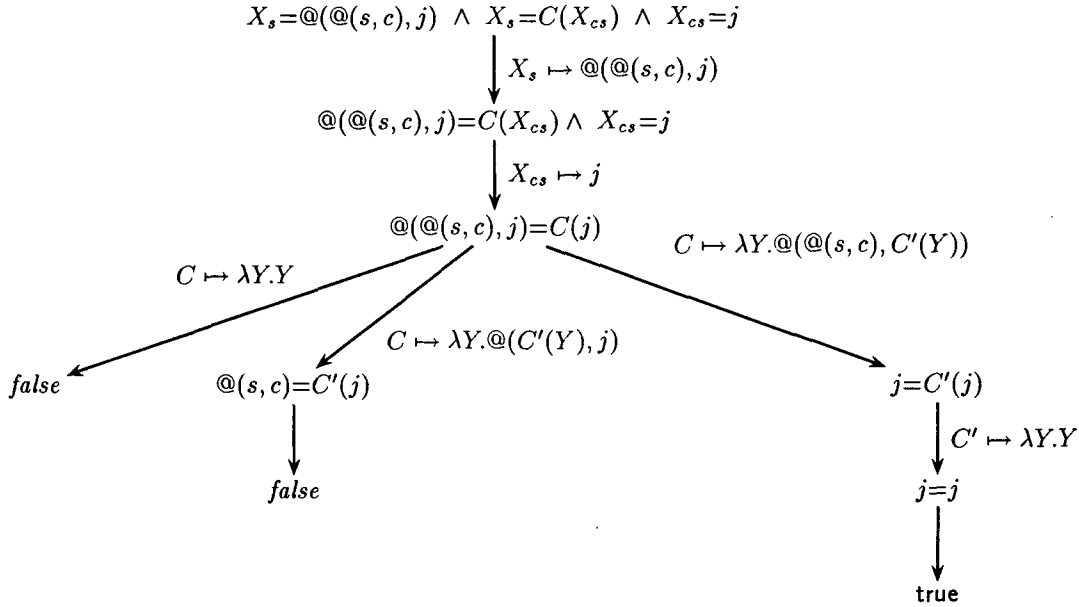
Figure 2: Solving the context constraints of example (11)(i)
