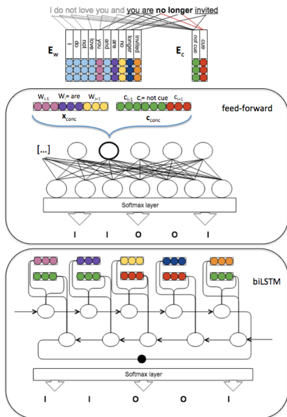
Figure 1: An example of scope detection using feed-forward and BiLSTM for the tokens ‘ you are no longer invited ’ in the instance in ex. (3b).
