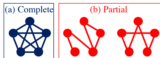
Figure 2: If we need training data for a graph labeling task (assuming the gold values for the nodes are given) and our annotation budget allows us to annotate, for instance, 10 edges in total, we could (a) completely annotate one graph (and then we run out of budget), or (b) partially annotate two graphs.
