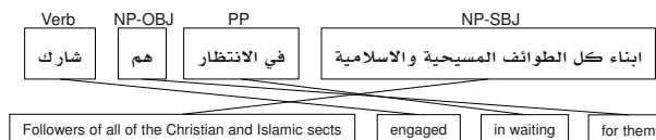
Figure 1: The oracle translation for this Arabic VOS sentence would be pruned during search using typical distortion parameters. The Arabic phrases read right-to-left, but we have ordered the sentence from left-to-right in order to clearly illustrate the re-ordering problem.
