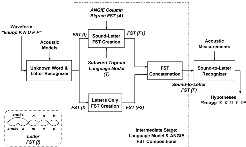
Figure 2: A schematic illustrating the multi-stage speak and spell recognition procedure. I , capturing the first stage letter hypotheses, is input to an intermediate stage, where F_1 (see steps 1 to 3 in Section 3.2.2) is concatenated with F_2 (step 4). The result F defines the search space for the final stage.
