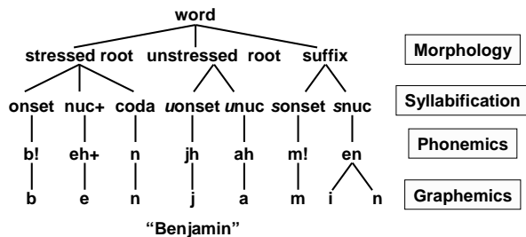
Figure 1: An example ANGIE parse tree for the word “Benjamin.”
