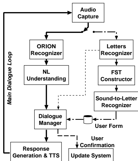
Figure 3: A schematic depicting the multi-threaded implementation for the speak and spell system.
