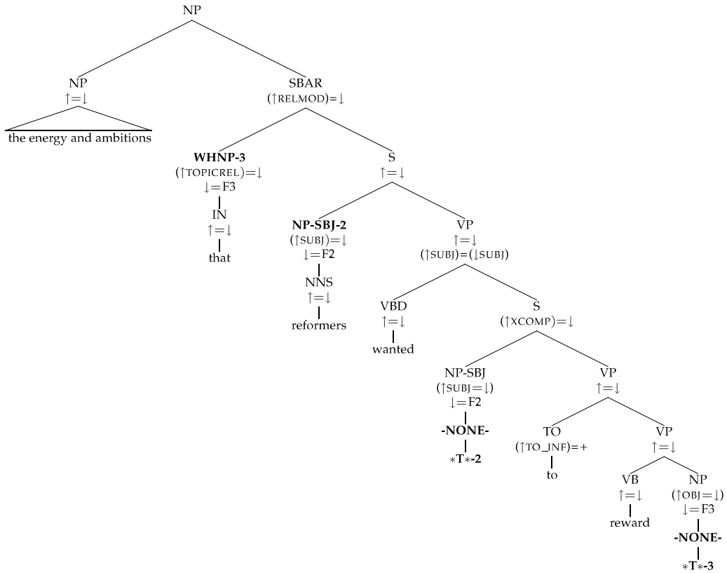
Figure 8 Penn-II treebank tree with LDD indicated in terms of traces (empty productions) and coindexation and f-structure annotations generated by the annotation algorithm.
