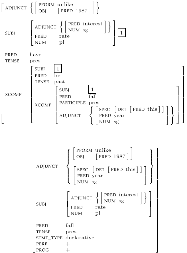
Figure 15 DCU 105 and PARC 700 analyses for the sentence Unlike 1987, interest rates have been falling this year.
