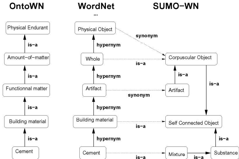
Figure 4: Cement example
