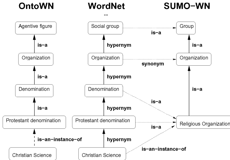
Figure 3: Christian_Science example
