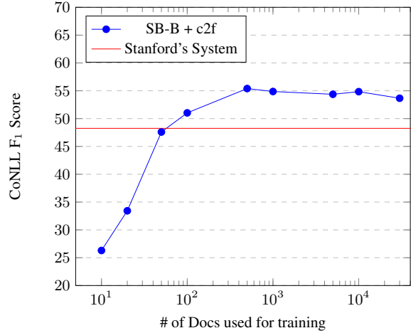
Figure 1: Performance on a held-out set of 1000 PreCo documents using the c2f-coref model as the number of documents used for training varies.
