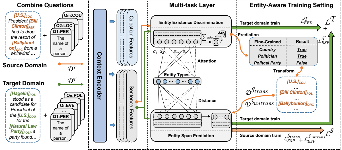
Figure 2: The Domain-specific entity-aware framework (DoSEA) for cross-domain NER. DoSEA has three components: a context encoder, a multi-task layer and an entity-aware training setting. There are different training processes for source and target domains.
