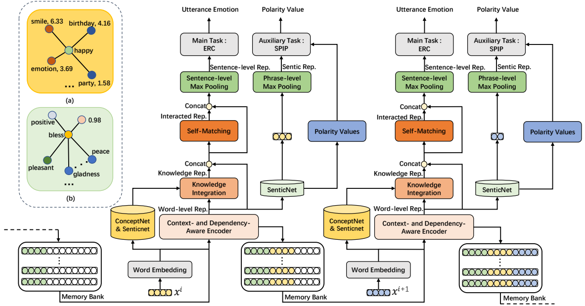
Figure 2: Overall architecture of our model. Rep. denotes representation. (a) is a sub-graph extracted from the ConceptNet with the keyword “happy” while (b) is an example provided by the SenticNet with the keyword “bless”.
