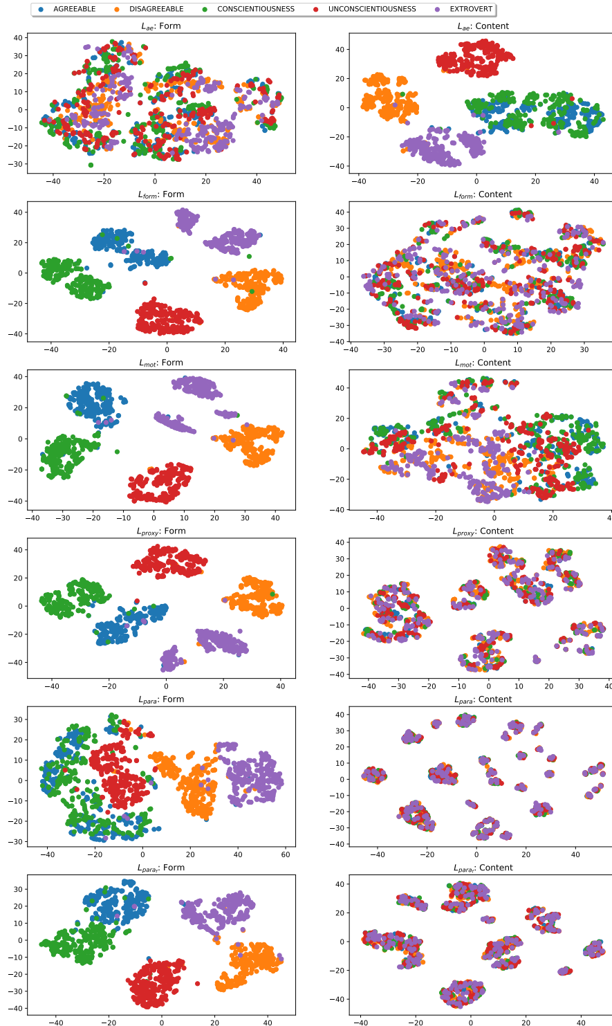
Figure 2: t-SNE visualization of form and content vectors for the PersonageNLG dataset, for each of our models. We see that the paraphrase losses enable a clean clustering of the meaning representations across stylistic variations. The domination of extrovert (purple) in some of the conditions is an artifact of the visualization when points fall in the same place.
