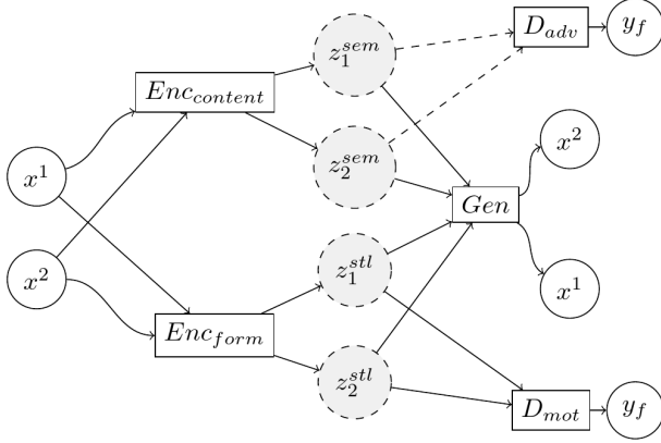
Figure 1: The main components of a Disentangled Representation Learning model. z^{sem} and z^{stl} denote the content and form vectors respectively; each is input to a motivational and an adversarial network. The generator is trained to reconstruct the original input as well as paraphrases.
