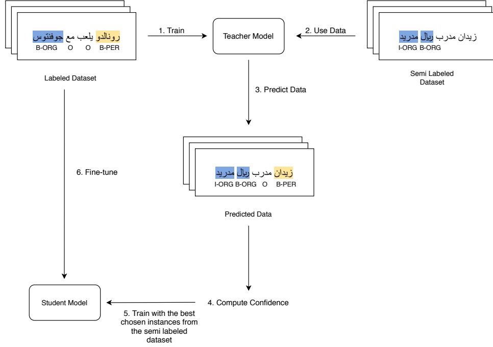
Figure 3: Semi-Supervised Learning Approach
