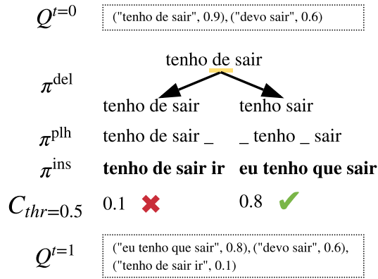
Figure 2: An example of a step of the inference algorithm of the paraphrasing model. A translation is taken from the queue \mathcal{Q} and expanded using LevT policies. Results are scored by the classifier C ; the translations scoring above the threshold thr = 0.5 are accepted. The translations are grounded in the source sentence by the encoder output.
