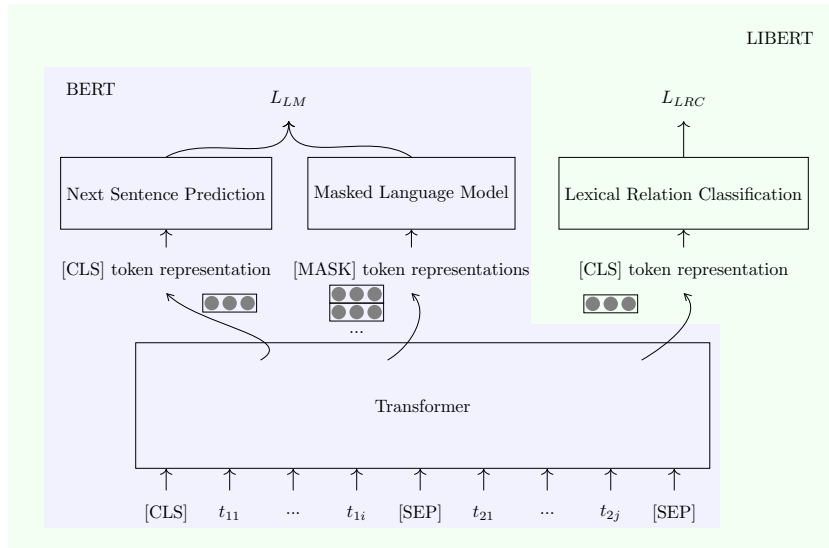
Figure 1: Architecture of LIBERT, lexically-informed BERT specialized with lexical similarity constraints.
