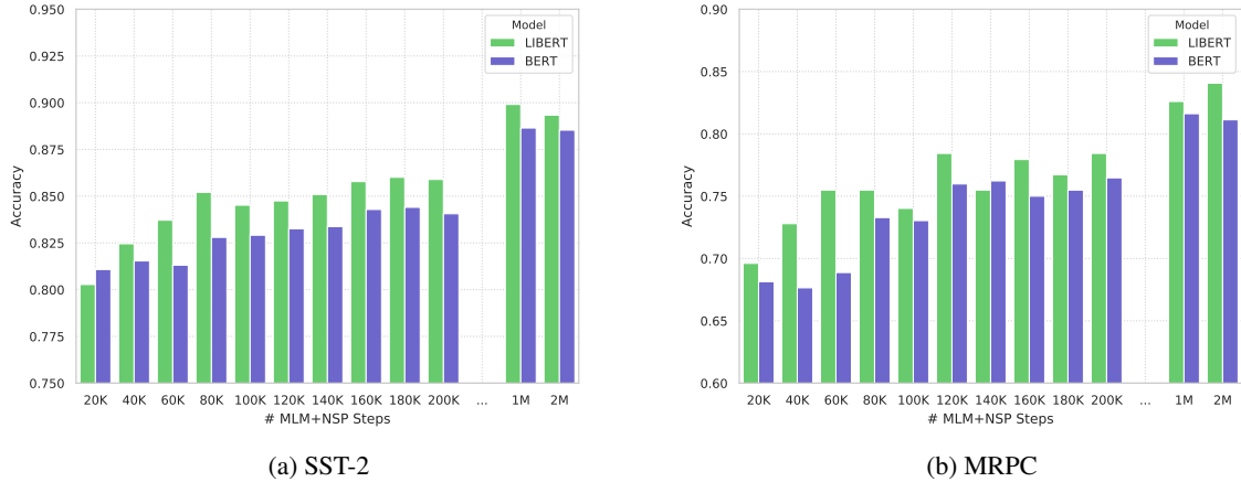
Figure 2: Accuracy over time for BERT and LIBERT on (a) SST-2 and (b) MRPC on the corresponding development sets.
