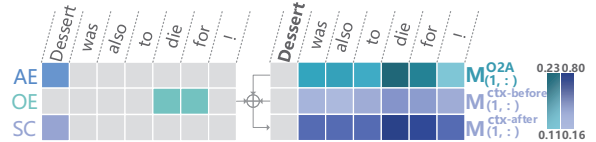
Figure 4: Visualization of the example S3.
