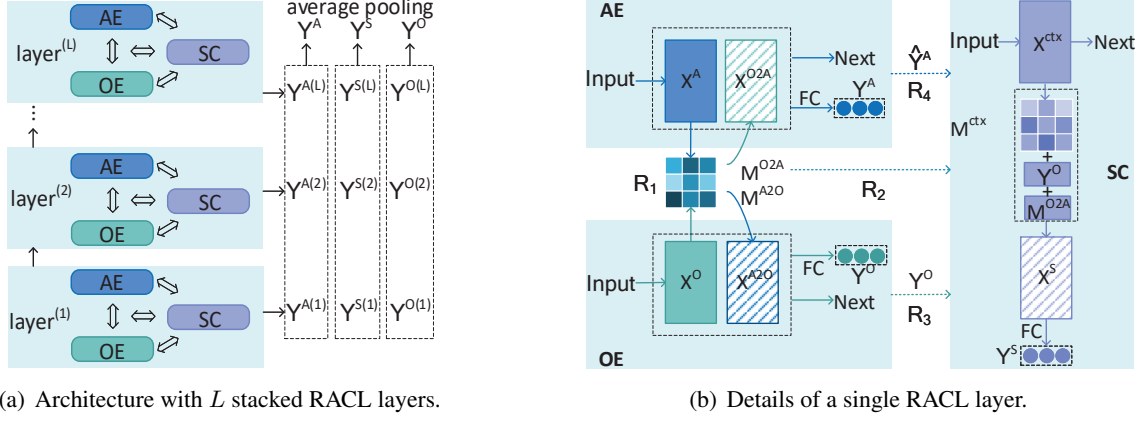
Figure 2: The proposed RACL framework.
