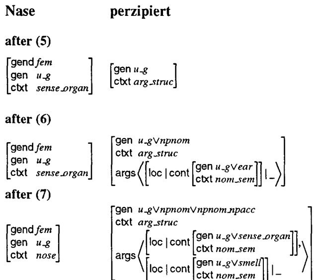
Figure 2: Updates on lexical FSs
