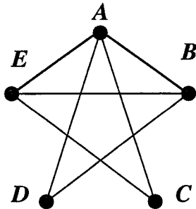
Figure 1: The decomposable model ABD.ABE.ACE . Edges of the separators, AB and AE (corresponding to ABD \cap ABE and ABE \cap ACE ), are drawn thicker. A separator is a set of vertices whose removal disconnects the graph.
