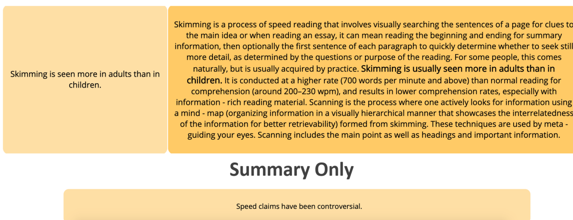
Figure 1: The interface of Margin Call displays summaries generated for each paragraph, allowing the user to decide to view the summary with the text it is generated from or by itself.
