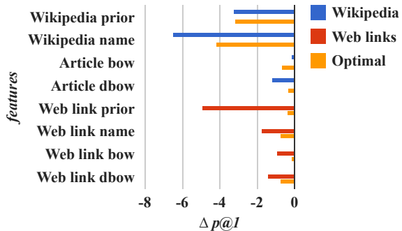
Figure 3: Ablation analysis of best configurations.
