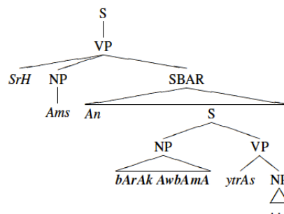
Figure 1: Example for the head word and syntactic environment feature
