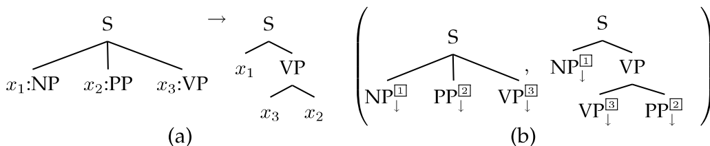
Figure 3 Two equivalent representations of the first rule in Example (5): (a) tree transducer; (b) Synchronous Tree Substitution Grammar (STSG). The ↓ arrows denote substitution sites, which correspond to variables in tree transducers.
