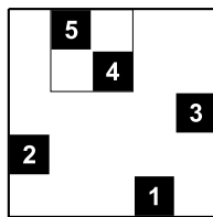
Figure 7 Example of Algorithm 1 on the non-binarizable input (2, 5, 4, 1, 3).
