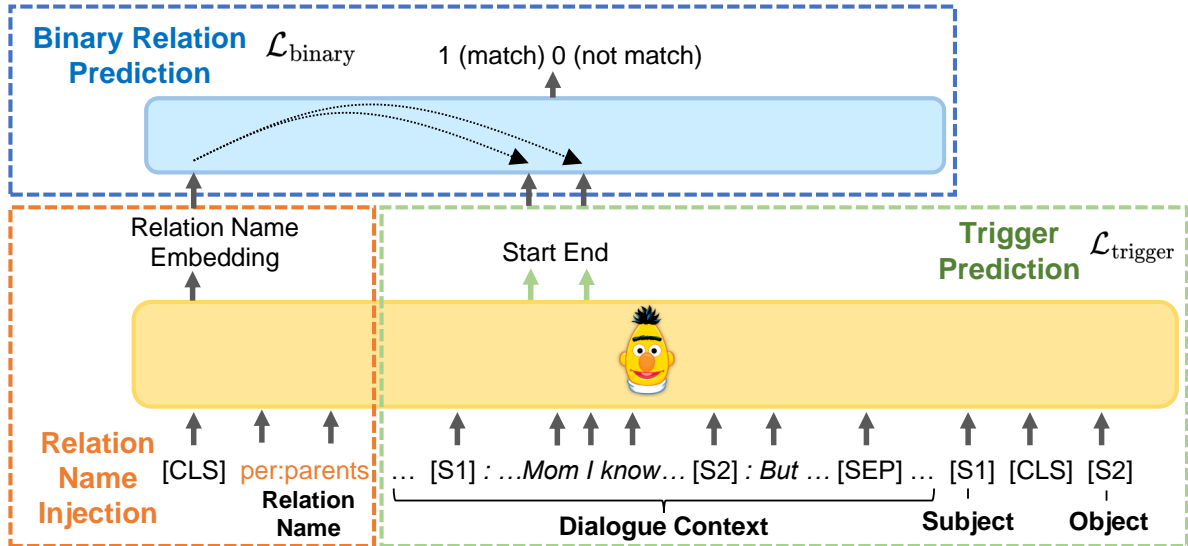
Figure 2: The illustration of our proposed model architecture.
