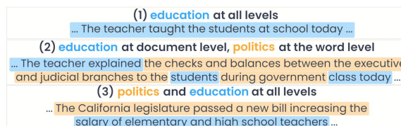
Figure 1: These are the three document types featured within a corpus. While existing methods can only distinguish between (1) and (3), MEGClass addresses all three types as well as minimizing (3) from the constructed pseudo-training dataset.
