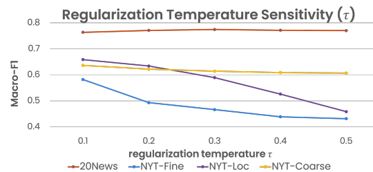
Figure 6: Sensitivity of the temperature scaling value for the weighted regularized contrastive loss. Macro-F1 scores are computed after the first iteration.
