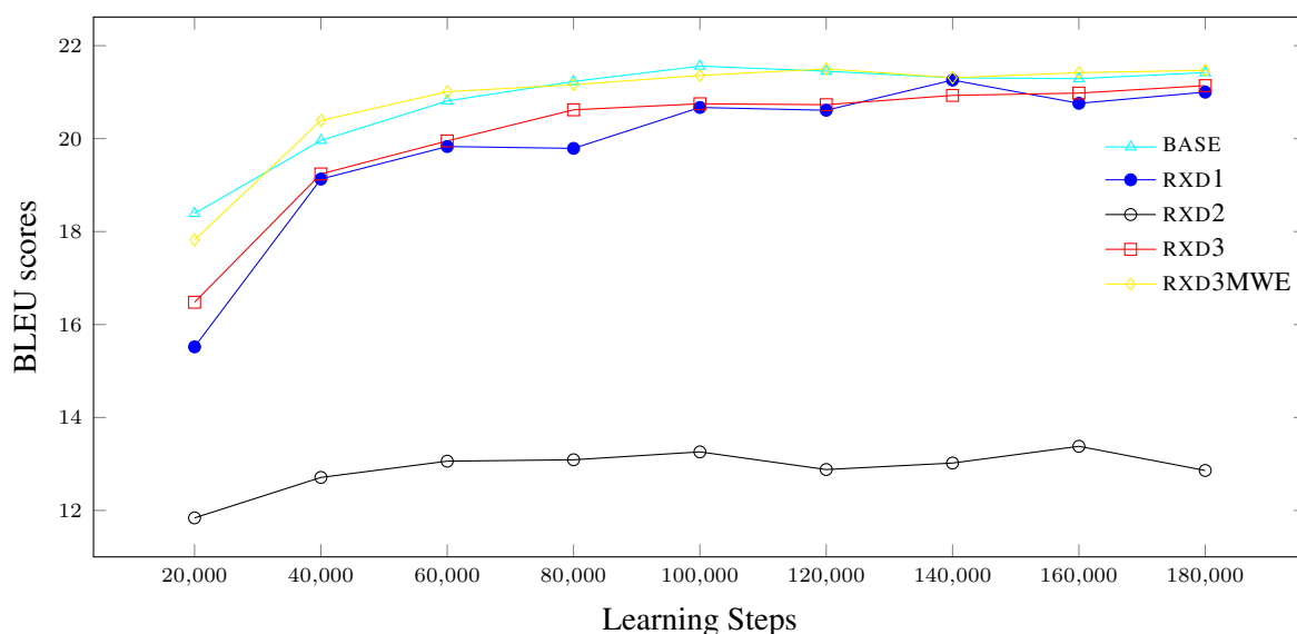
Figure 6: Learning curves from different models with BLEU metric
