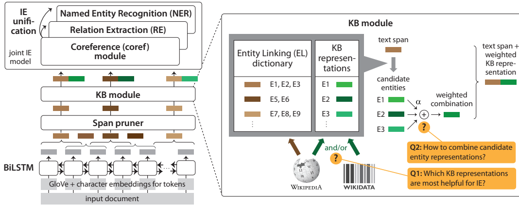
Figure 1: Joint information extraction (IE) model with addition of a knowledge base (KB) module.
