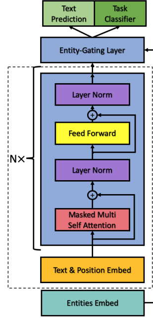
Figure 1: CoreLM Architecture as an extension of GPT2 model (area within dashed border).
