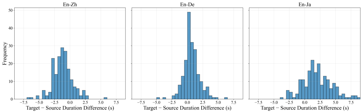
Figure 2: Distribution of target-source duration differences on the ACL 60/60 dev set. En→Zh is mostly negative, En→De is centered around zero, and En→Ja is mostly positive.
