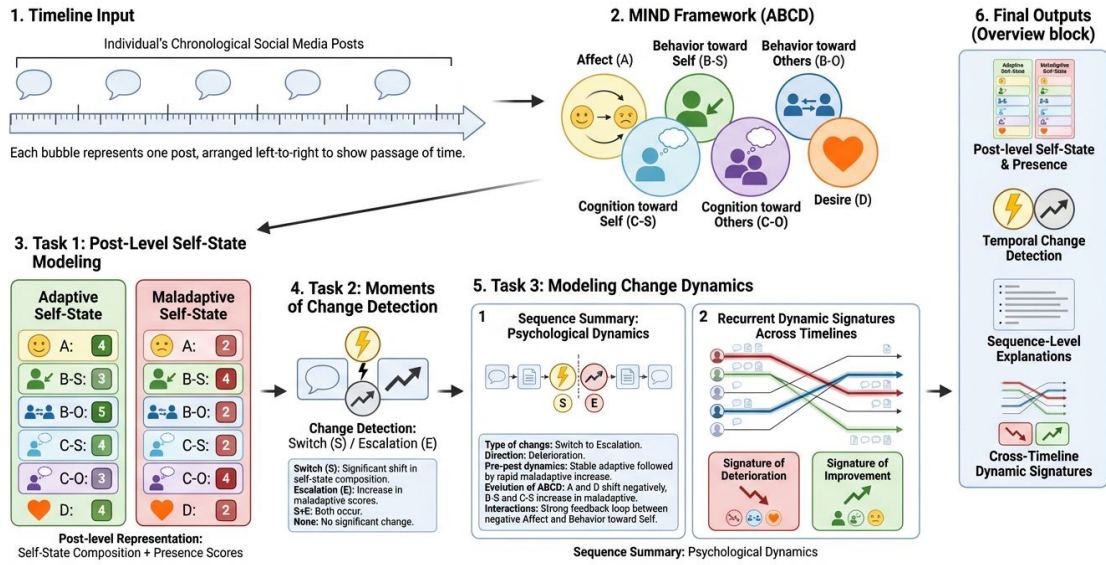
Figure 2: Illustration of the CLPsych 2026 shared task pipeline for modeling mental health dynamics from longitudinal social media timelines. The framework maps chronological posts to adaptive and maladaptive self-states using the MIND (ABCD) model, followed by detection of moments of change (switches and escalations) and sequence-level modeling of deterioration/improvement dynamics. Final system outputs include post-level self-state predictions, temporal change detection, sequence summaries, and cross-timeline mental health signatures.
