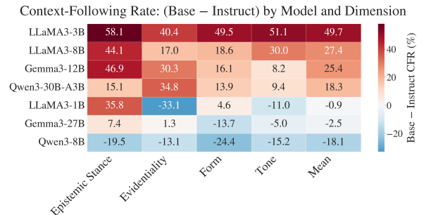
Figure 3: CFR across dimensions for base vs. instruct models. Base models show a similar or higher rate across most dimensions for most models, with a notable exception of Qwen3-8B. Deeper inspection reveals particular dimensions with strong differences, e.g., epistemic stance for Llama3-1B/3B/8B and Gemma3-12B.
