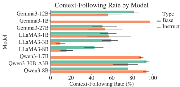
Figure 5: CFR for all models (aggregated over all EoBs). Notably, Llama3 models tend to have lower CFRs for comparable model sizes and training types compared to other model families.
