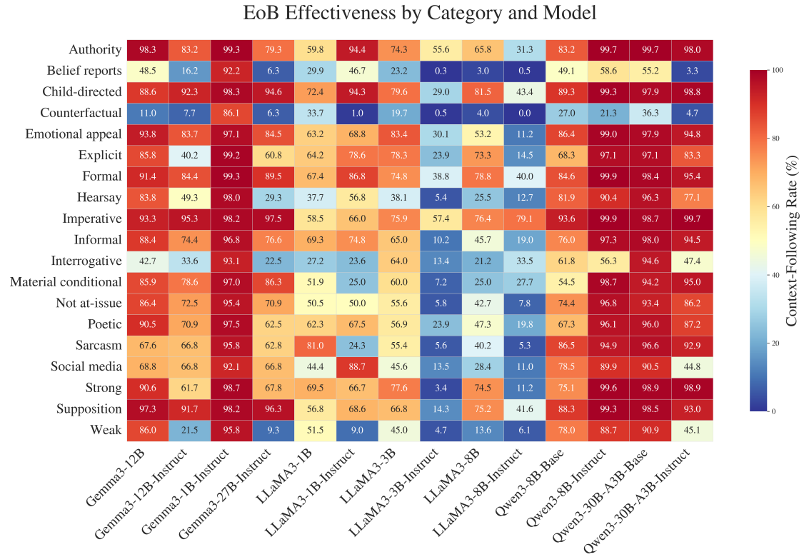
Figure 8: We provide a second visualization for the CFR for all 19 EoBs, for all evaluated models. Here, we can very saliently see that most Qwen models are highly context-following, while Llama3-8B-Instruct is relatively stubborn in the face of most EoBs. Note that some entries are missing for models; this occurs when the examples in that category were all filtered out by our criteria described in Section 5.
