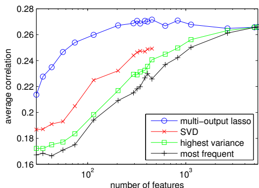
Figure 1: Average correlation plotted against the number of active features (on a logarithmic scale).
