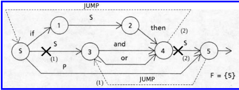
Figure 7 Turning recursions into iterations.
