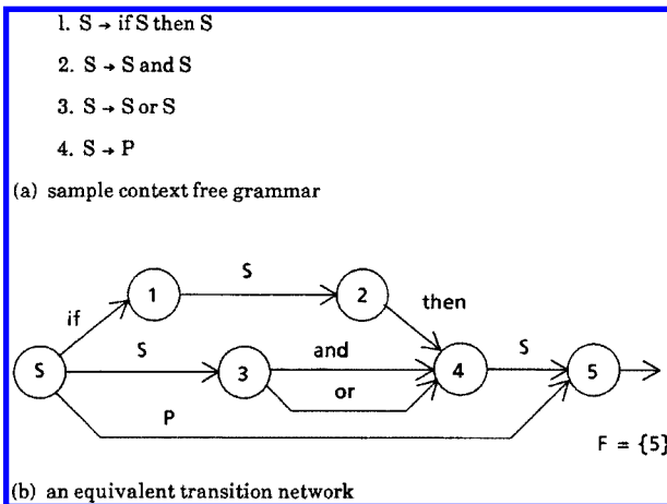
Figure 6 Factoring the common parts of rules.
