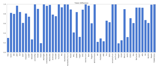
Figure 2: fraction of token occurrences (of 50 most frequent tokens) in the discarded data
