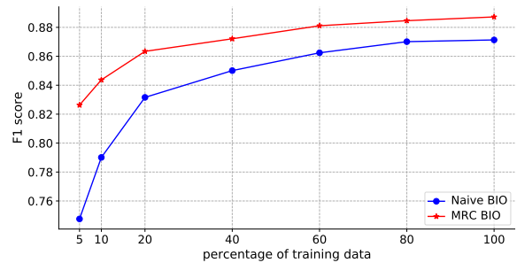
Figure 4: F1 score under different percentages of data on CoNLL2005 development set.
