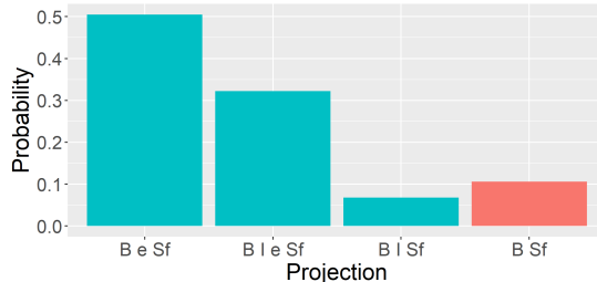
Figure 1: Probability distribution over projections of B I e S_f . Ungrammatical projections are colored red. val_{(\pi_P, G)}(B I e S_f) = 0.895 , which is the sum of the probabilities of the grammatical projections. Note that the probability of a particular projection is independent of whether or not it is grammatical: here, ungrammatical B S_f has a higher probability of being projected than grammatical B I S_f .
