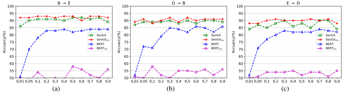
Figure 3: The influence of sample number. We explore the influence of sample number with different rate of source domain. For the limited space, we only show the results of B → E, D → B, and E → D.
