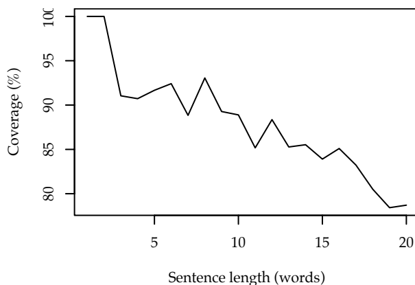
Figure 5. Proportion of sentences for which the parser finds (among all its parses) a fully correct dependency structure, per sentence length
