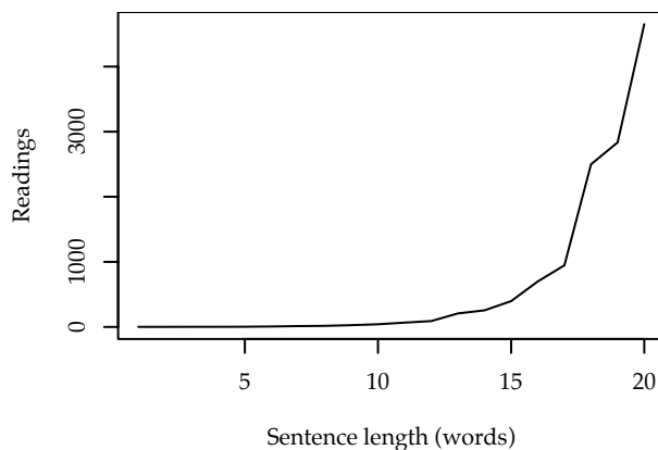
Figure 4. Mean number of parses per sentence length
