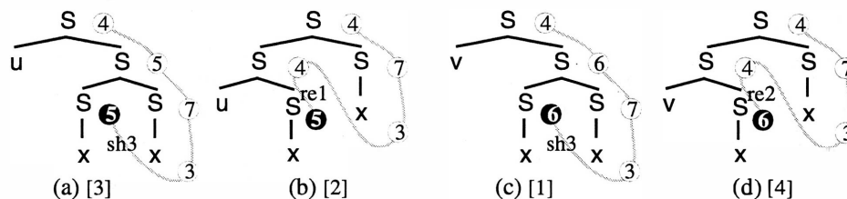
Figure 3. Training set (The square-bracketed number below each tree denotes the number of occurrences of that tree.) parameters 4 .
