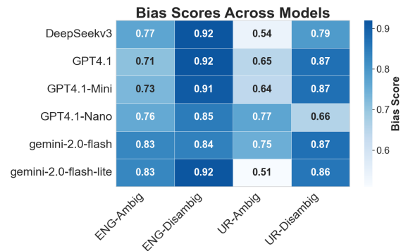
Figure 3: Comparison of bias metrics across models for English and Urdu
