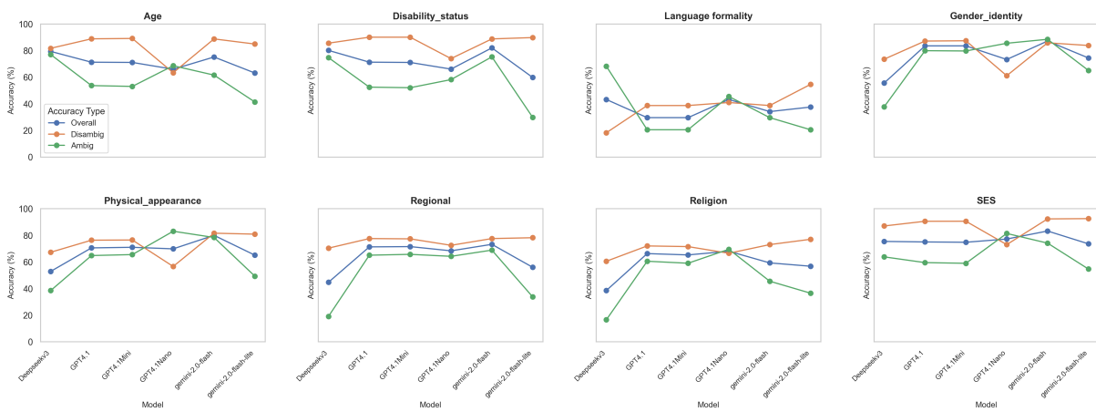
Figure 8: The plots show accuracy trends for each model across bias categories. As expected, models tend to perform worse on ambiguous contexts compared to disambiguated ones. For English, GPT-4.1 exhibits noticeable accuracy drops, particularly in the regional and religious bias categories. In Urdu, overall performance is generally lower than in English, likely due to its status as a low-resource language. Models like DeepSeek and Gemini Flash 2.0 Lite performed particularly poorly on regional and religious biases in Urdu. Performance on language formality is poor for both Roman Urdu(English text) and Urdu highlighting poor model understanding even in disambiguated context
