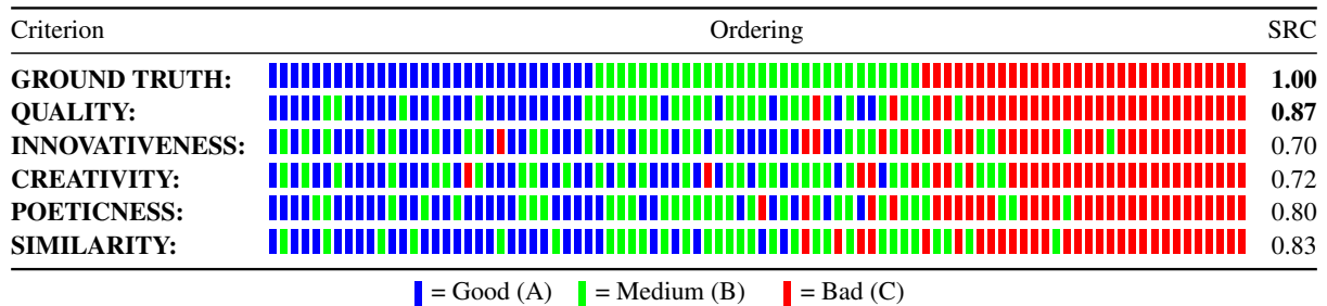
Figure 2: Poem orderings generated by Claude-3-Opus 15n, the best-performing model and method from Experiment 3 (Section 7.3). The results demonstrate a strong correlation with the ground truth, with the “Quality” criterion achieving a Spearman’s Rank Correlation (SRC) of 0.87—a significant improvement over the best human non-expert evaluation (SRC = 0.38, see Figure 1).
