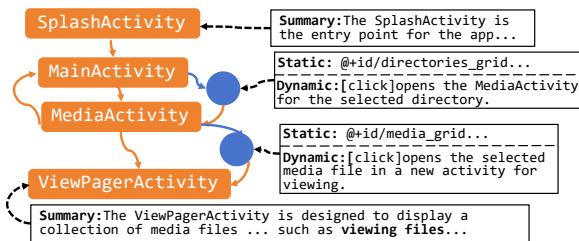
Figure 2: Part of the UI Map of the app named Gallery.
