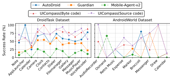
Figure 4: Success Rate across Different Apps
