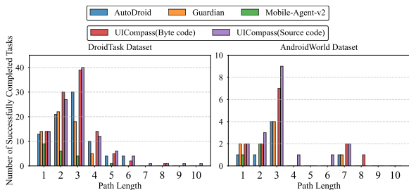
Figure 5: Success Rate across Different Path Length.
